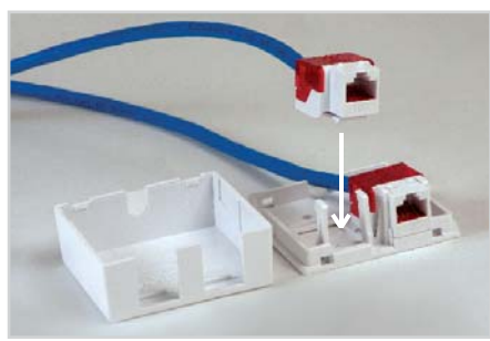
Install connectors tab-side down
