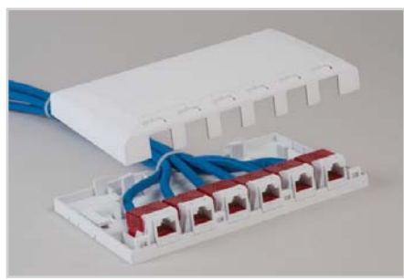
Removable cover
